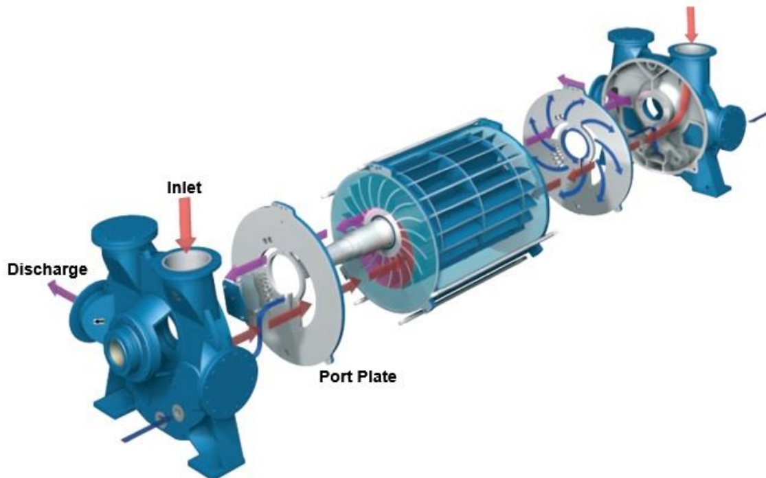
Flat Plate Type Vacuum Pump (Exploded View)
